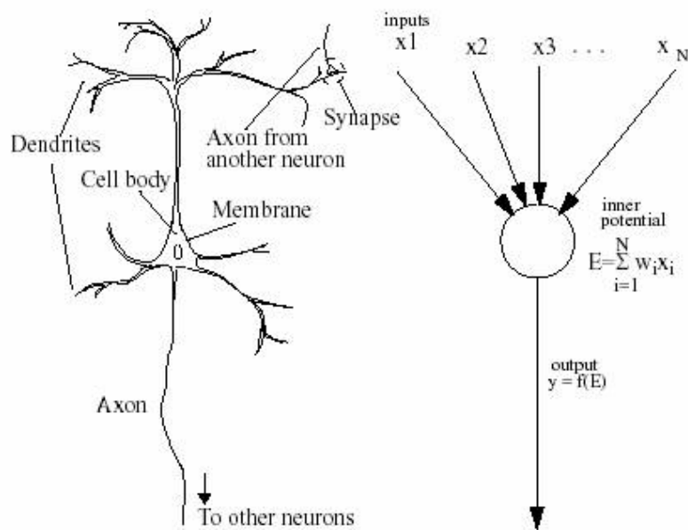
Figure 2.5: BNN/ANN Analogy
