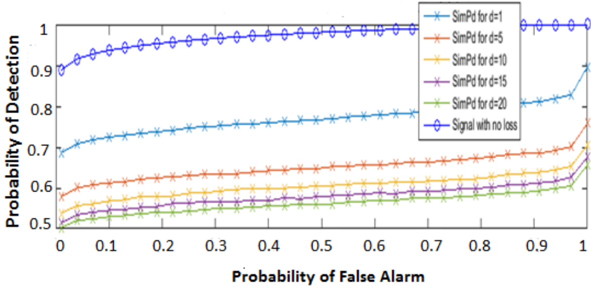
Figure 4.4: Sensing performance with different path loss values (different distances)
