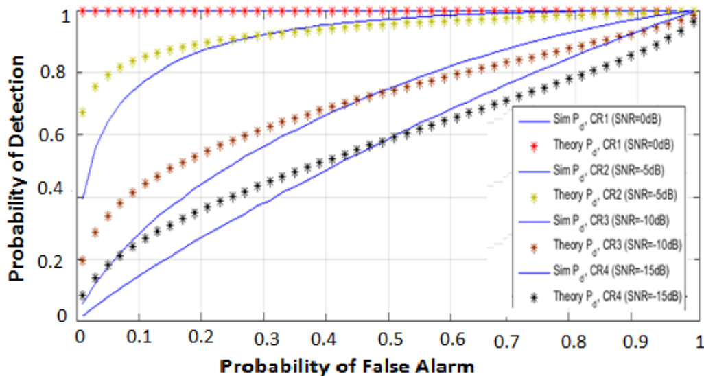
Figure 4.2: ROC Plot for Multiple SUs with different SNR values
