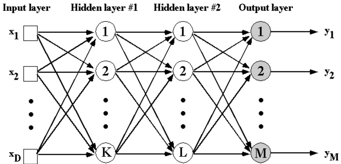
Figure 3.7: Multilayered Perceptron ANN
