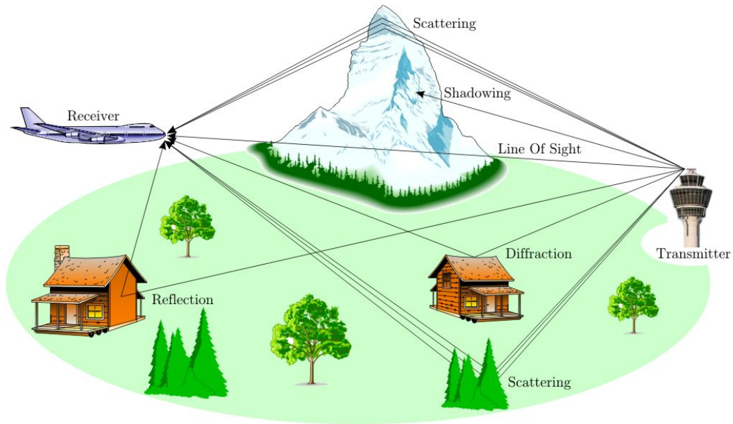
Figure 2.2: Channel Impairments
