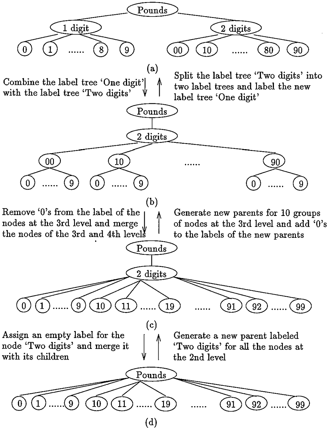
Figure 3.1: The transformations between implicit and explicit structures.
