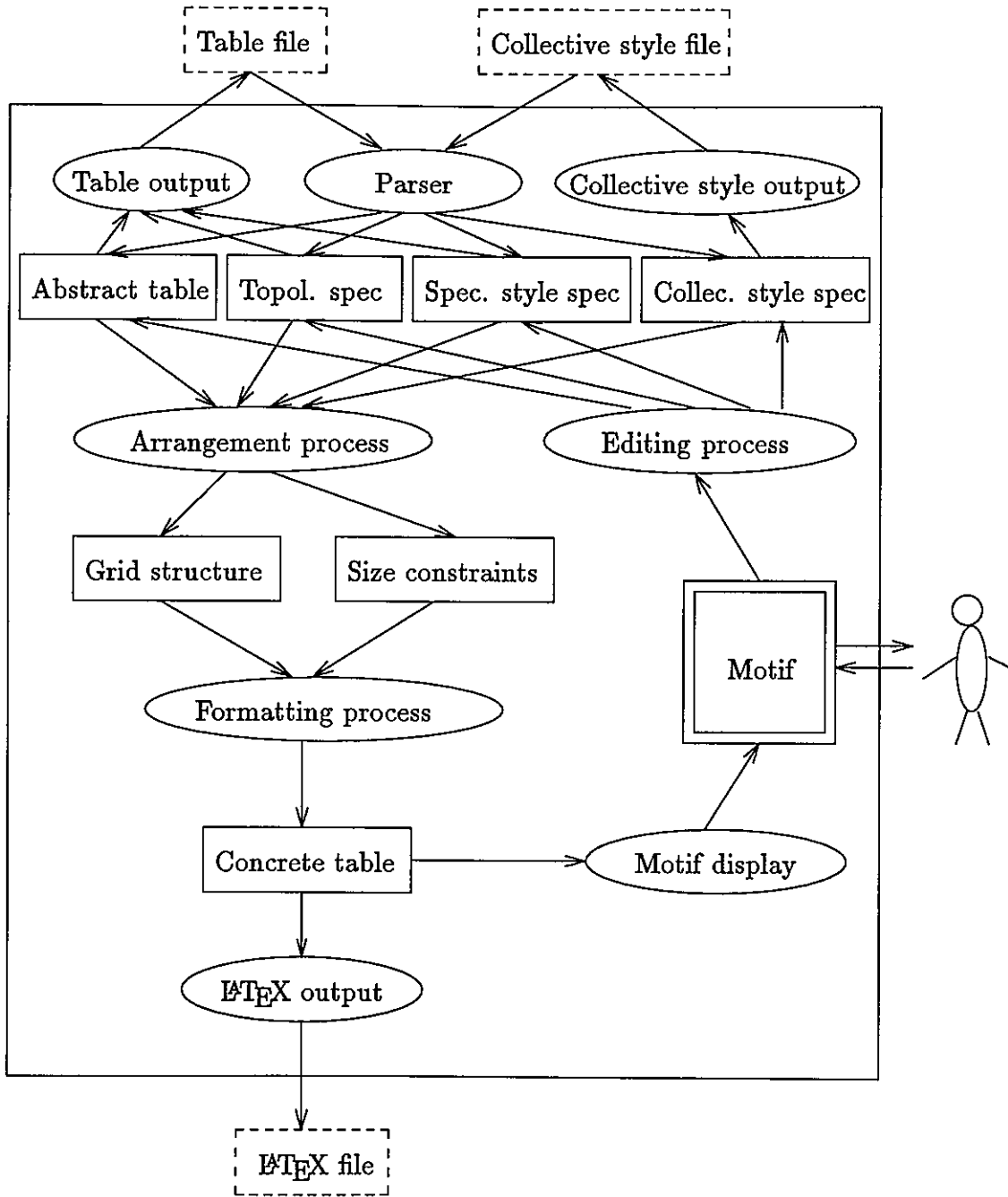
Figure 6.4: The internal system structure of XTABLE.
