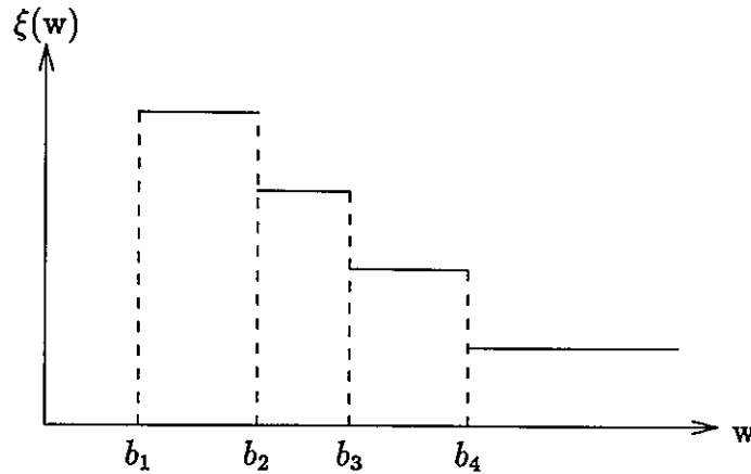
Figure 5.2: The characteristics of a size function.
