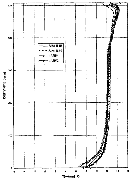
Figure 6 Temperature profiles, IGU 6, clear triple 12.7 mm foam spacer.
