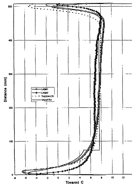
Figure 9 Simplified models vs. measured temperature profiles, IGU 2.
