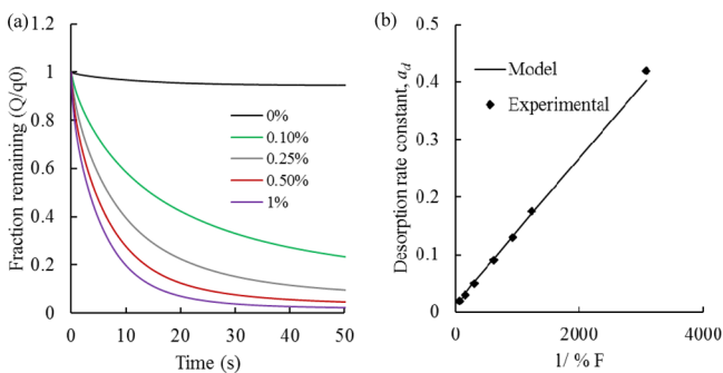
Figure 6. (a) Effect of matrix concentration on desorption kinetics in finite volume case. K_{es} = 100 , K_a = 1 \times 10^5 L/kg, k_d = 1 s -1 (labile). (b) The dependence of desorption rate constant, a_d , on the free concentration of pyrene present in sample with increasing concentration of a binding matrix (BSA). The free concentration of analyte decreases with the addition of BSA in the sample.
