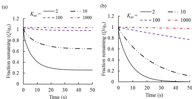
Figure 1. Fractions of calibrants remaining on the extraction phase at different partition coefficients ( K_{es} ) (a) finite sample volume, flow velocity = 0 cm s -1 and (b) infinite sample volume with flow velocity of 0.1 cm s -1 . For both the cases, the absence of a binding matrix component is assumed. Coating thickness was 45 μm; D_s ( 7.33 \times 10^{-6} cm 2 s -1 ) was considered for all the calibrants so that \delta_s does not vary by the compound, D_e = D_s/6 .
