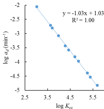
Figure 3. Desorption rate constant, a_d , obtained by varying the coating-sample partition coefficient ( K_{es} ) by keeping all other conditions the same as Figure 1.
