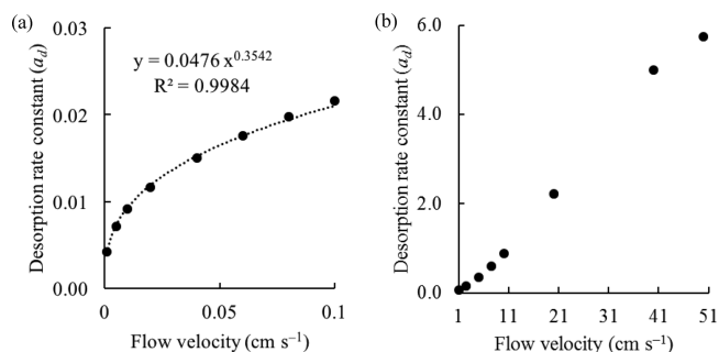
Figure 4. Dependence of a_d as a function of linear sample flow velocity at two flow regimes: (a) laminar flow and (b) turbulence flow. Model simulation was carried out by using \log K_{es} = 4 , D_s = 1 \times 10^{-6} cm s -1 .
