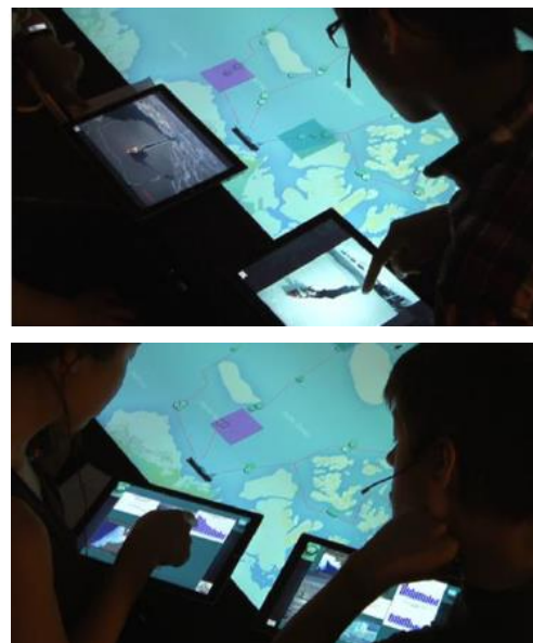
Figure 5. Groups 11 (top) and 10 (bottom) forming tableaux
