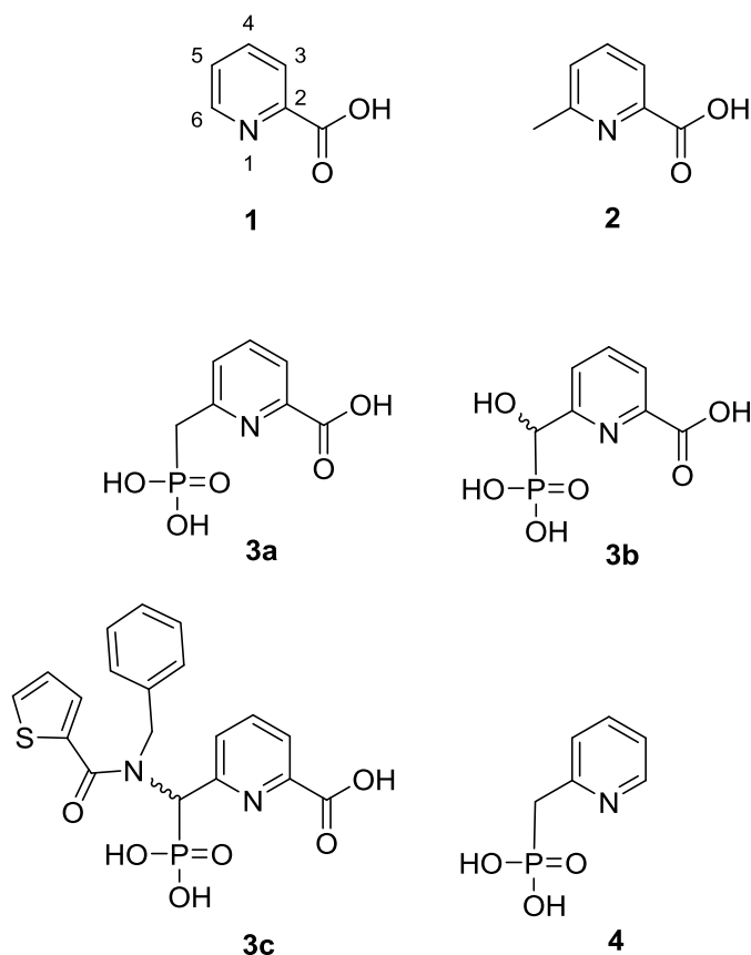
53 Figure 1. Structures of pyridine-2-carboxylates used in this study. 1, PA, 2-picolinic acid; 2, 54 MPA, 6-methylpicolinic acid; 3a, PMPC-1, 6-(phosphonomethyl)pyridine-2-carboxylate; 3b, PMPC- 55 2, 6-[hydroxy(phosphono)methyl]picolinic acid; 3c, PMPC-3, 6-[(N-benzyl-1-thiophen-2- 56 ylformamido)(phosphono)methyl]picolinic acid; 4, (pyridin-2-ylmethyl)phosphonic acid.
