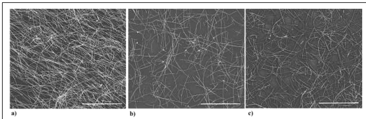
Figure 33: SEM images of a suspension of Ag124 deposited by a) spin Coating, b) Mayer rod coating and c) spray coating. Scale bar = 100 μm.
