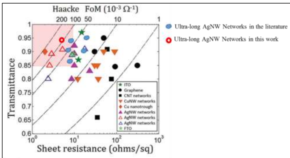
Figure 38: Transmittance (550 nm) plotted as a function of sheet resistance for various transparent conductive materials reported in the literature: ITO, graphene, single-walled carbon nanotubes, copper nanowires, silver nanowires, FTO and the present work. [18]
