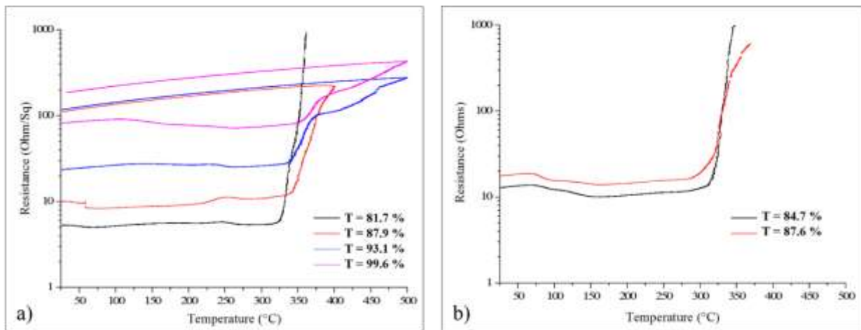
Figure 36: Plots of the resistance measured in-situ versus temperature during thermal ramp ( 5^{\circ}\text{C}/\text{min} ) of electrodes made with a) Ag135 and b) Ag101 at different initial resistances and transparency presented in table 2.4.
