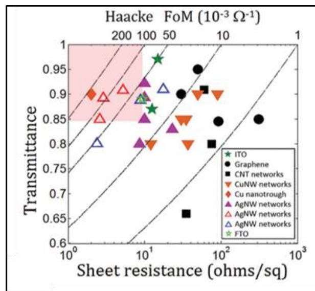
Figure 4: Transmittance (550 nm) plotted as a function of sheet resistance for various transparent conductive materials: Indium tin oxide (ITO), graphene, single-walled carbon nanotubes, copper nanowires, silver nanowires, and FTO. The solid lines are associated with iso-values of the Haacke FoM (Figure of Merit). [18]
