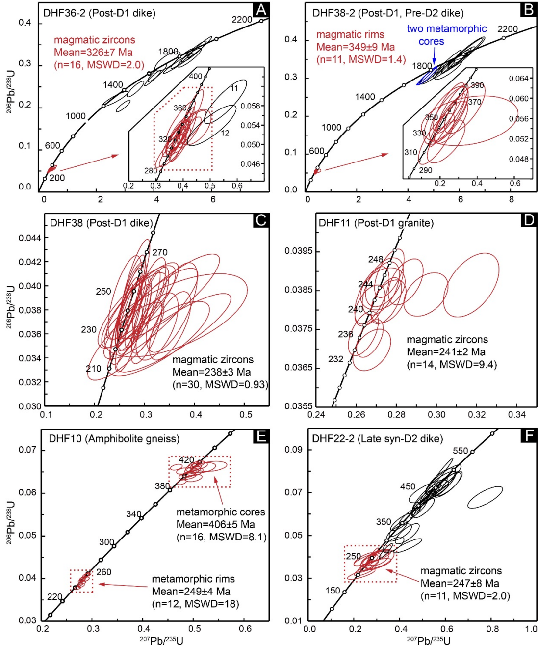
Figure 12. Zircon U–Pb concordia diagrams
