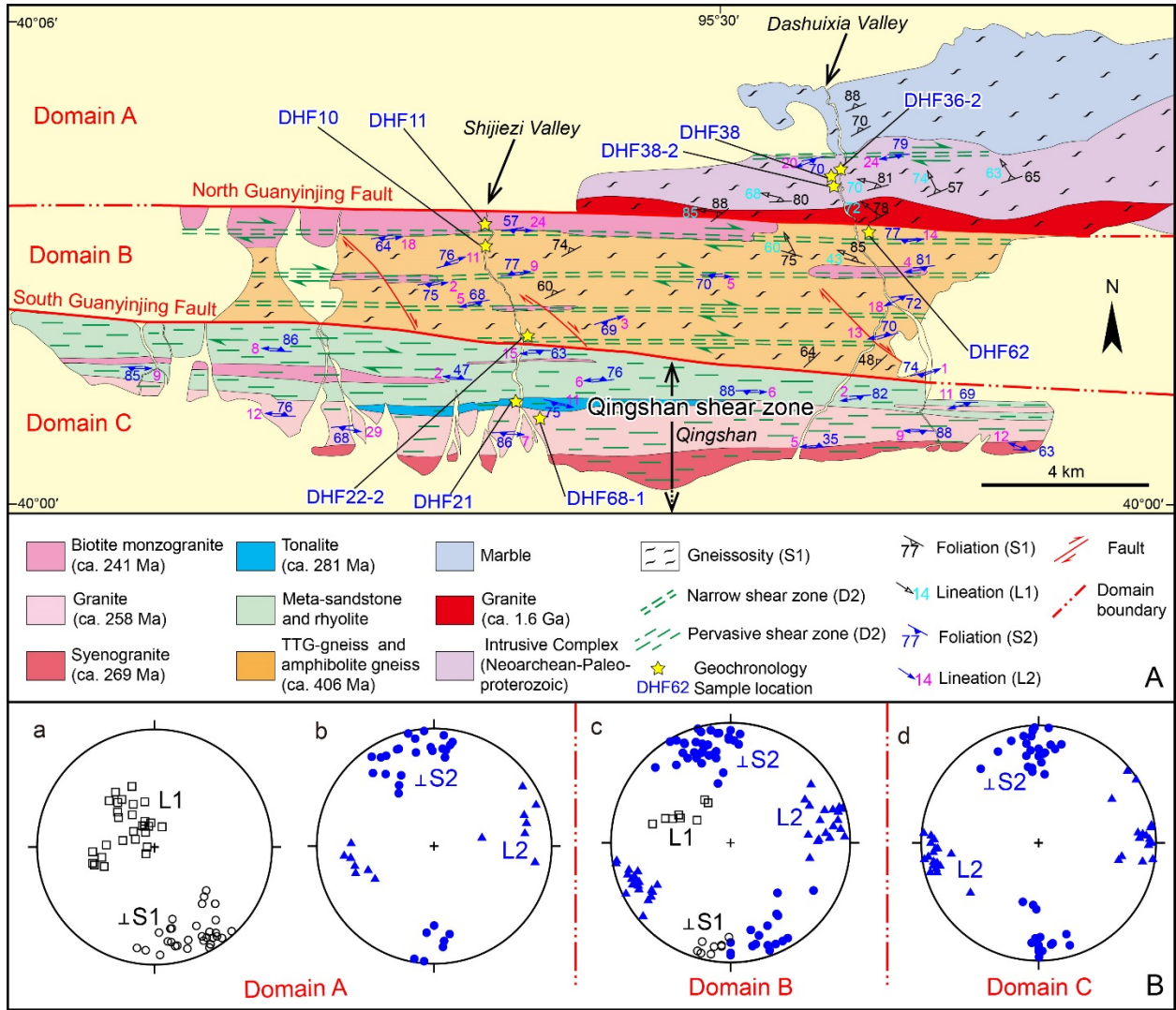
Figure 3. A: Geological map of the Dashuixia valley–Qingshan area. Geochronology sample locations are indicated by yellow stars; B: Equal-area lower-hemisphere projections of poles to foliation (S) and stretching lineation (L).
