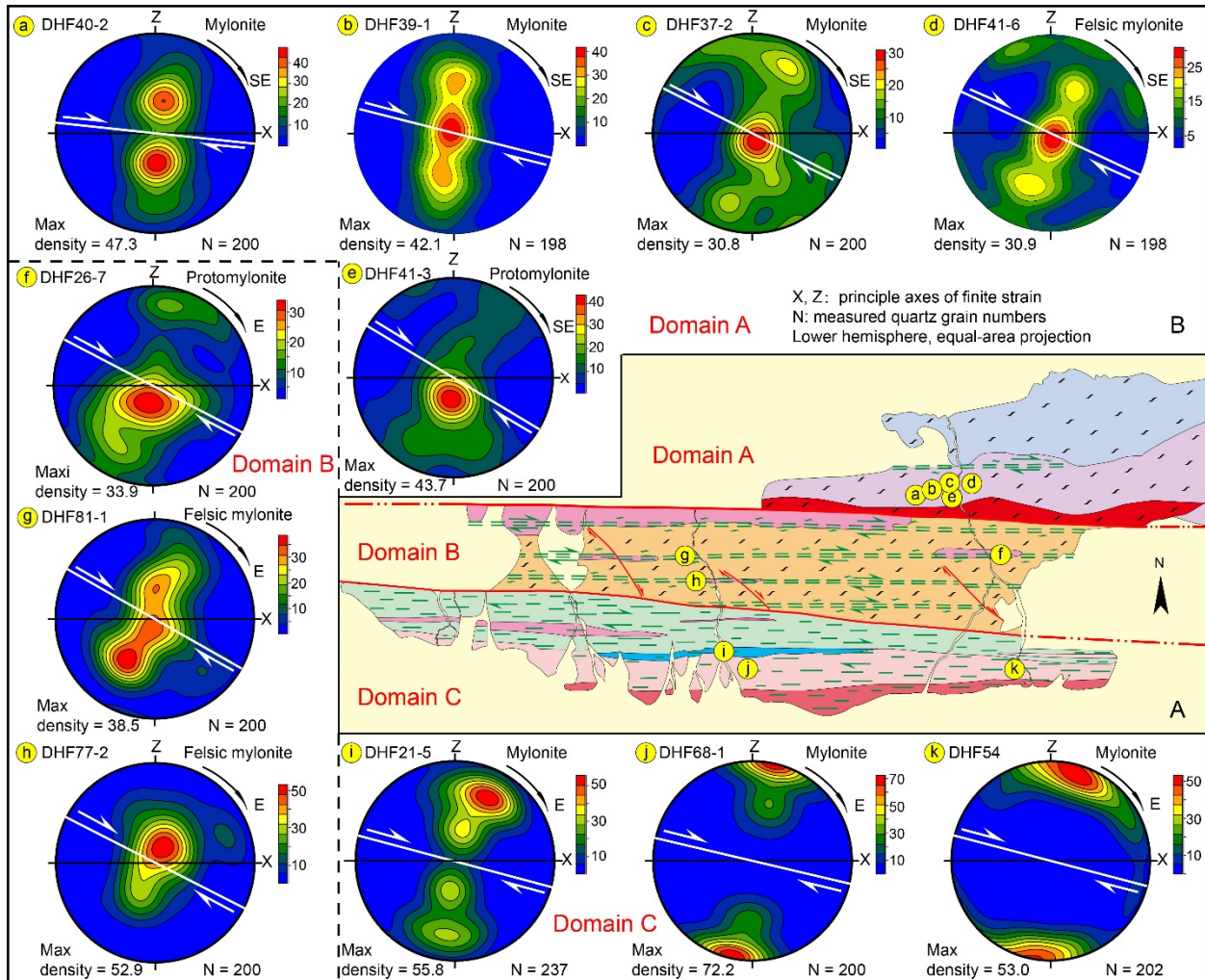
Figure 9. Equal-area, lower-hemisphere projections of C-axes of recrystallized quartz grains measured by U-stage. All sections are parallel to the stretching lineations. The patterns indicate top-to-SE shearing in domain A and dextral strike-slip shearing in domains B and C. The number of measurements in each sample is also shown.
