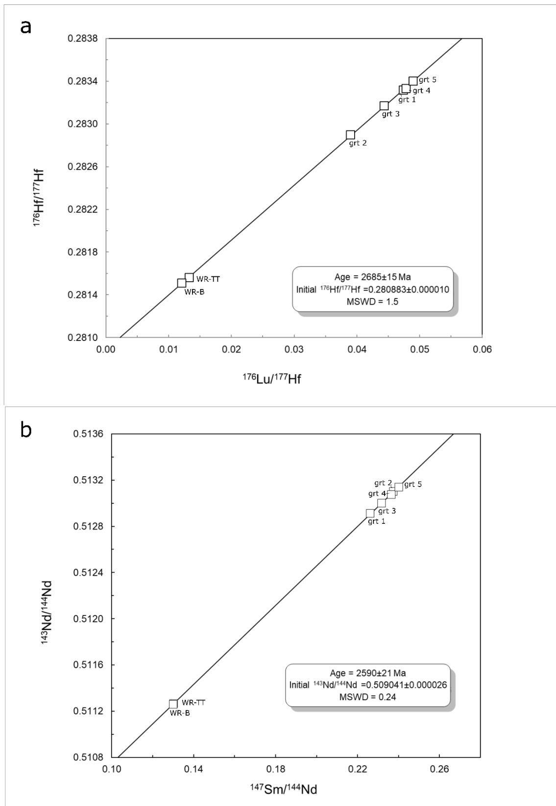
Figure 3.16. Garnet Lu-Hf (a) and Sm-Nd (b) isochron diagrams for sample 229151. Uncertainties are 2\sigma . ( WR-TT : whole-rock table top; WR-B : whole-rock bomb).
