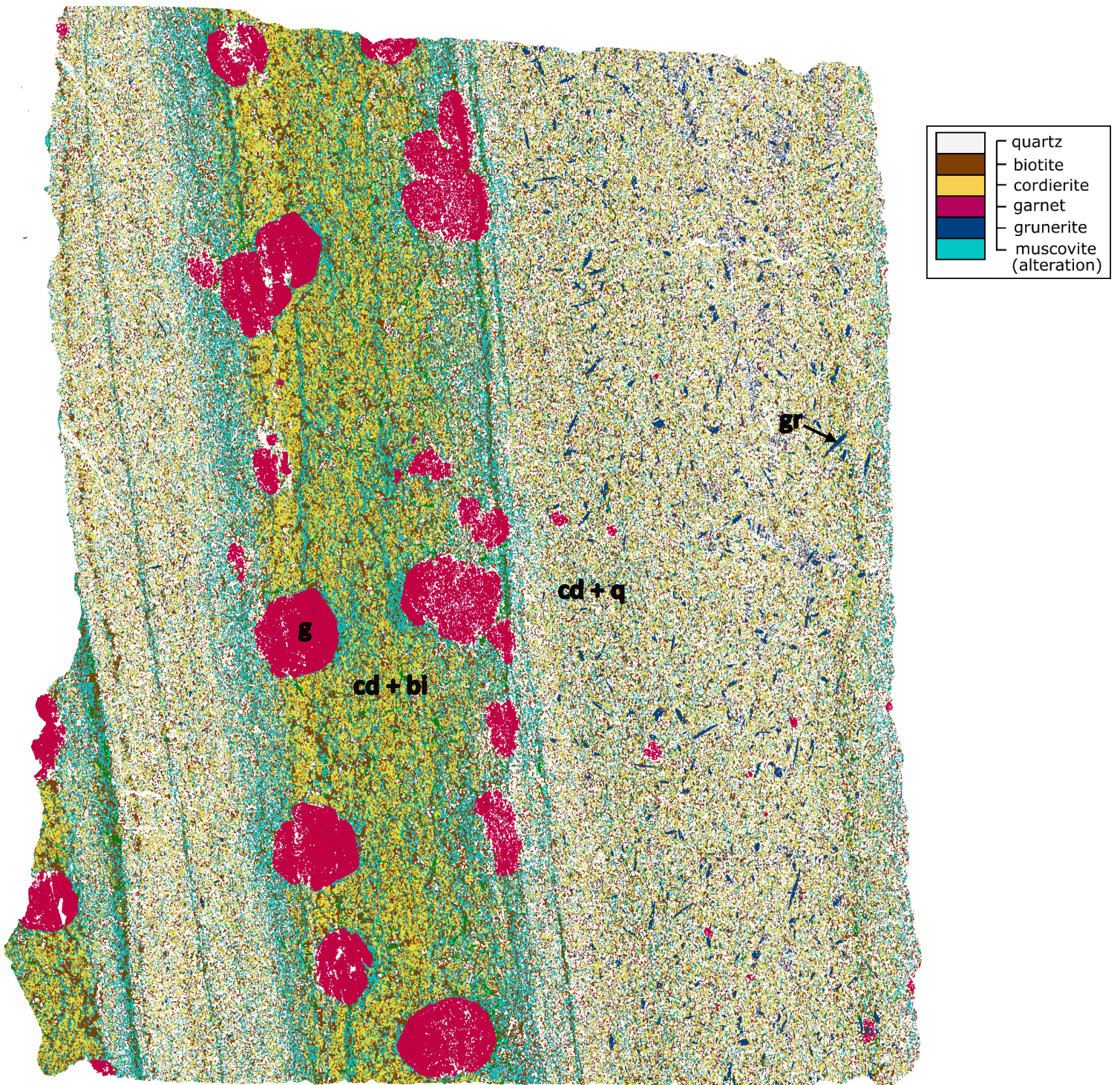
Figure 3.6. SEM-MLA false coloured map of sample 229120 showing compositional layering, with the first layer displaying blue grunerite porphyroblasts within a matrix of quartz and minor cordierite, and the second layer showing large garnet porphyroblasts within a matrix of cordierite and muscovite alteration. The false coloured map was made of a thin section that is 2.5cm x 2cm in size.
