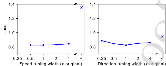
Figure 7: Validation loss of gesture recognition networks as a function of speed-tuning width (left) and direction-tuning width (right). The horizontal axis is as in Figure 6. For example, 1 indicates the original speed-tuning width distribution, and 2 indicates that the scale parameter of the distribution was increased by a factor of two. The points on the right (marked with x) indicate infinite tuning width (i.e. no sensitivity).
