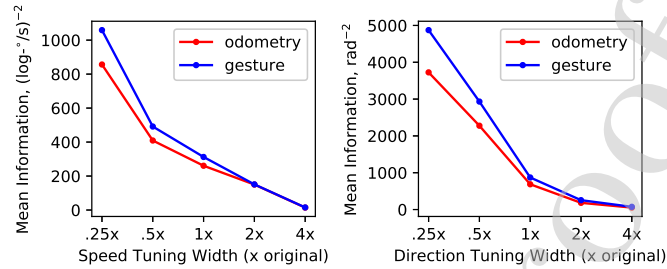
Figure 8: Left, Fisher information about log-speed, for MT model populations with different speed-tuning widths. The red and blue lines correspond to the odometry and gesture recognition tasks, respectively. These are slightly different because the Fisher information is calculated as a weighted average over the actual speed distributions that appeared in these tasks. The task-specific direction distributions were ignored, because direction tuning was statistically uniform. Right, Fisher information about direction, for MT model populations with different direction-tuning widths.
