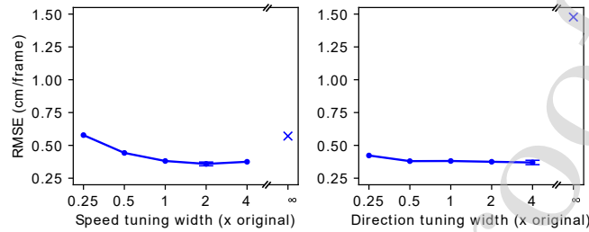
Figure 6: Root-mean-square error of odometry predictions on held-out validation data, as a function of speed tuning width (left) and direction tuning width (right). The standard deviation of the targets was 1.54. On the horizontal axis, 1 means the distribution is unchanged, 2 means the scale parameter of the Gamma distribution is 2x its original value, etc. The error bars indicate \pm 2 SD for repeated training with different random initialization.
