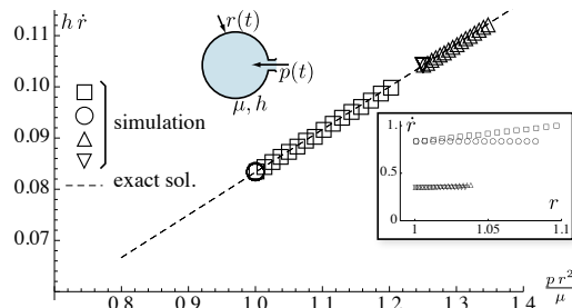
Figure 6: Validation of stretching, based on the inflation of a viscous, spherical balloon under internal pressure p(t) . Four simulations were run, indicated by different shapes ( \triangle \nabla \square \circ ). These correspond to a sheet of thickness h = .1 and viscosity \mu = .1 ( \square \circ ) or to h = .3 and \mu = .1 ( \triangle \nabla ), and to a time-independent pressure ( \square \triangle ) or to a decreasing pressure p(t) proportional to 1/r^2 ( \circ \nabla ), where r is the current sphere radius. In inset, raw data are shown in the plane (r, \dot{r}) . In the main plot, the same data is shown in terms of rescaled coordinates x = p r^2 / \mu and y = h \dot{r} , and compared to the exact solution y = x/12 .
