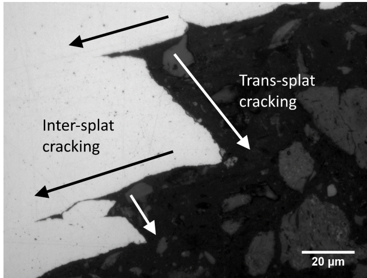
Figure 24. OM image of inter-splat and trans-splat cracking along fracture surface cross-section
