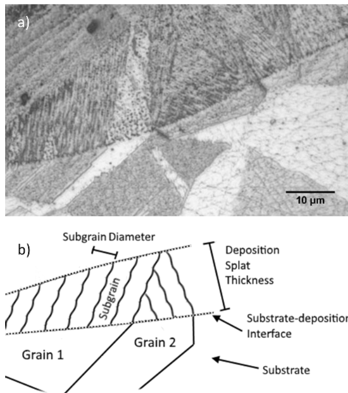
Figure 11. a) OM image along substrate-deposition interface and b) schematic of competitive cellular dendritic subgrain growth directions at the interface
