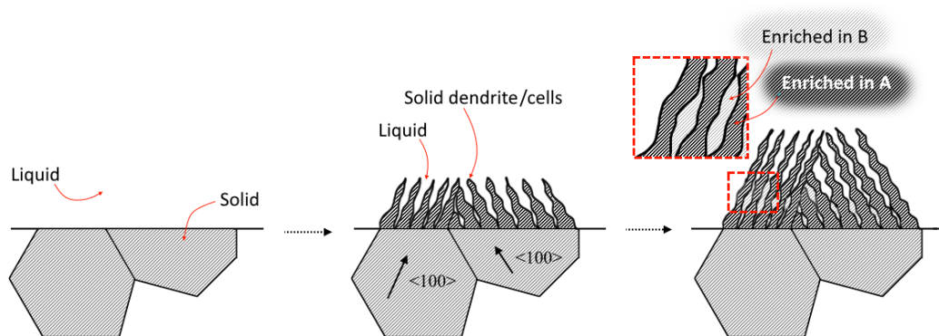
Figure 7. Schematic depiction of cellular dendritic growth from two substrate grains and micro-segregation at the cell boundaries
