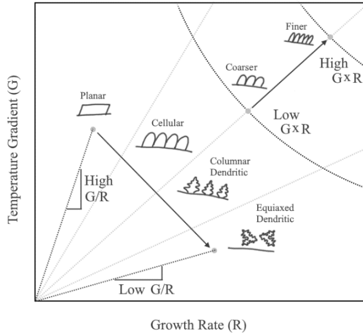
Figure 6. Solidification microstructure depending on temperature gradient and growth rate, adapted from [58,59]
