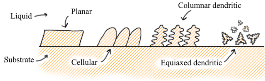
Figure 5. Depiction of planar, cellular, columnar dendritic, and equiaxed dendritic solidification microstructures
