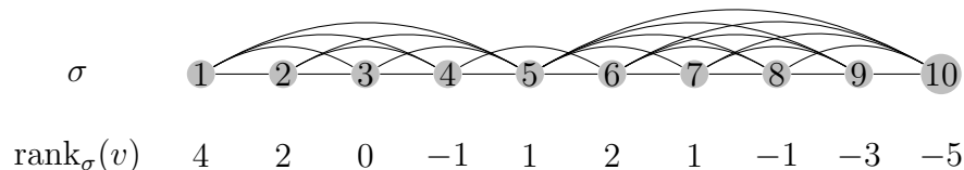
Figure 4.12: A proper interval graph with diameter 2 which does not satisfy the requirements of Lemma 3.4.2. Note that the ordering is a regular ordering, and that it is imbalance-minimal.
