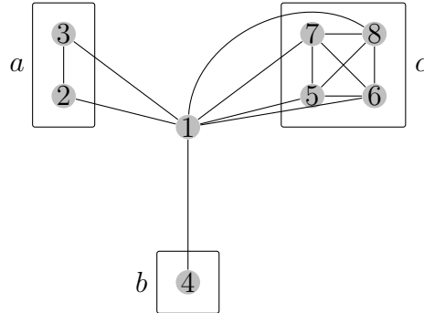
Figure 4.10: A superfragile graph G illustrating how the FPT algorithm for IMBALANCE fails for tc(G) . The set T = \{1\} is a twin cover of G . Each of the disjoint cliques K_2 = \{3, 2\} , K_1 = \{4\} , and K_4 = \{5, 6, 7, 8\} are contracted into vertices a , b , and c respectively in G' .
