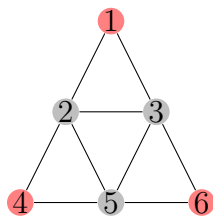
Figure 2.8: A graph with an asteroidal triple (1, 4, 6) .
