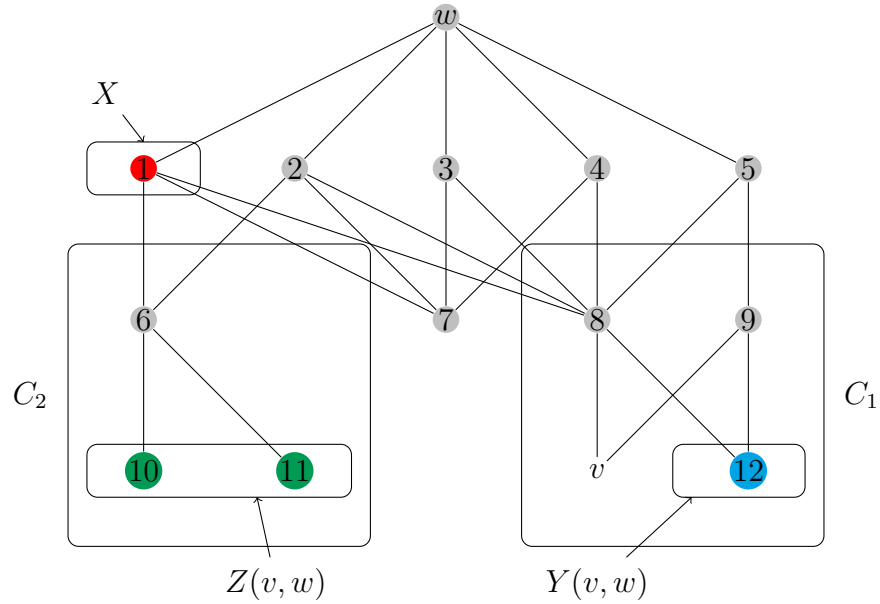
Figure 6.7: An example bipartite permutation graph with the sets used in Theorem 6.3.7 indicated. The deep components C_1 and C_2 of G - N[w] are indicated. The vertex v is a BFS end-vertex: \sigma = \langle w, 1, 2, 3, 4, 5, 6, 7, 8, 9, 10, 11, 12, v \rangle is a BFS ordering ending at v . The green vertices are the set Z(v, w) , the blue vertices are the set Y(v, w) , and the red vertex is the necessary set X(v, w) .
