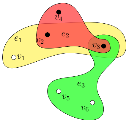
(a) A hypergraph H with a bisection \mathcal{B} of black-filled and white-filled vertices. Observe that \text{cost}(\mathcal{B}) = \text{cost}(e_1, \mathcal{B}) + \text{cost}(e_2, \mathcal{B}) + \text{cost}(e_3, \mathcal{B}) = 1 + 0 + 1 = 2 .
