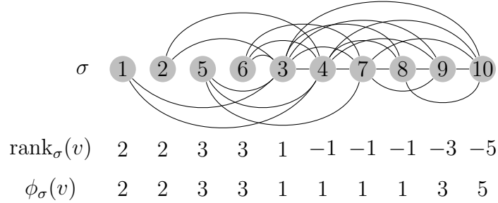
Figure 2.3: An illustration of the rank of a vertex.
