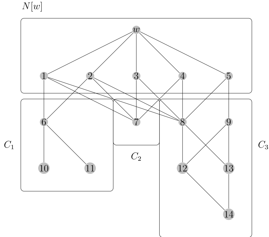
Figure 6.2: An illustration of the types of components considered in this work. The components of G - N[w] are C_1 = \{6, 10, 11\} , C_2 = \{7\} and C_3 = \{8, 9, 12, 13, 14\} . The components C_1 and C_3 are non-trivial components of G - N[w] , while the component C_2 is trivial. Since d(14, w) = \text{ecc}(w) = 4 , C_3 is also a deep component.
