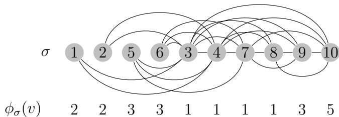
(b) An ordering \sigma of G such that im(\sigma) = 22 . By trying all possible permutations of V(G) , one can check that im(G) = 22 , and thus this ordering is imbalance-minimal.
