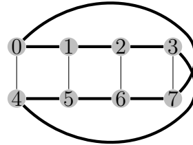
(b) The graph M_4 . Thick edges are cycle edges.
