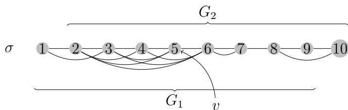
Figure 4.11: A proper interval graph G illustrating how to use induction for IMBALANCE. The vertices 1 and 10 can be considered the “ends” of the graph. The ordering \sigma is in fact imbalance-minimal, as is \sigma_{V(G_1)} and \sigma_{V(G_2)} , and all of these orderings are regular orderings. The vertices to the left of v (and v itself) have the same imbalance in \sigma_{V(G_1)} and \sigma , while the vertices to the right of v (and v itself again) have the same imbalance in \sigma_{V(G_2)} and \sigma . These vertices are indifferent to what happens at the other “end” of the graph. Putting \sigma_{V(G_1)} and \sigma_{V(G_2)} together by using the ordering G_1 \setminus G_2 \cdot G_1 \cap G_2 \cdot G_2 \setminus G_1 keeps those imbalances, and results in the ordering \sigma .
