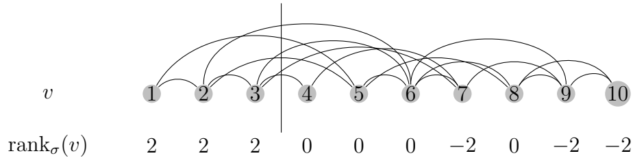
(b) An ordering \sigma such that cw(\sigma) = cw(T_3) . The vertical line is the first largest cut.
