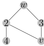
Figure 6.4: A vertex v of a bipartite permutation graph which is a BFS end-vertex but not an LBFS end-vertex.
