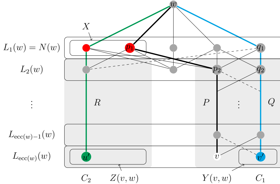
Figure 6.8: An illustration of the proof of Claim 6.3.8. Each layer may have more vertices than is shown. Regardless of other vertices, u' \in Z(v, w) is (one) vertex such that every set X \subseteq N(C_2) that separates u' and w must also intersect a shortest (v, w) -path. The paths P , Q , and R are not necessarily the only such paths, but are drawn to illustrate the important properties of each path. The graph is drawn so that the path P is always left of the path Q in C_1 to clearly illustrate that p_i is not adjacent to q_{i+1} . Similarly, there may be other choices for R , but in any case, q_1 is not adjacent to R \cap L_2(w) .
