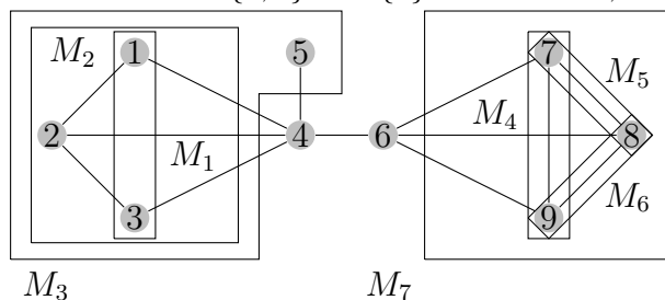
(b) A graph G with non-trivial modules M_1, M_2, M_3, M_4, M_5, M_6, and M_7 . Since G can be partitioned into modules M_3, \{4\}, \{6\}, M_7 and each of the graphs G[M_3] and G[M_4] have modular width at most 4, mw(G) = 4 .
