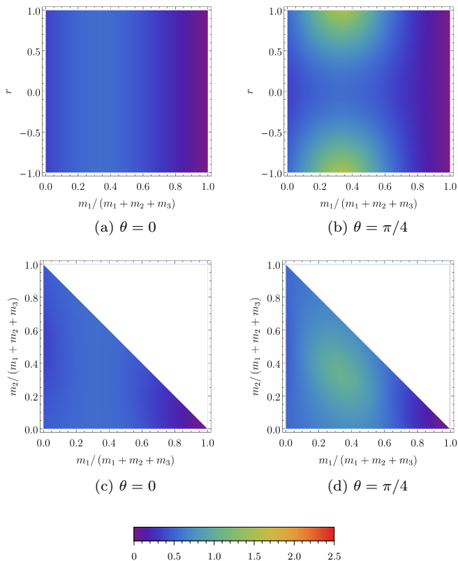
FIG. 5. (Colour online) The logarithmic negativity of the relative state of particles 2 and 3 described by \mathbf{V}_{23|1} is plotted, characterizing the entanglement among the relational degrees of freedom. In (a) and (b) the logarithmic negativity is plotted for the case m_2 = m_3 , for various equal phase rotations \theta_1 = \theta_2 = \theta_3 = \theta , as a function of the ratio m_1/(m_1 + m_2 + m_3) and equal squeezing parameters r_1 = r_2 = r_3 = r . In (c) and (d) logarithmic negativity is plotted as a function of the mass ratios m_1/(m_1 + m_2 + m_3) and m_2/(m_1 + m_2 + m_3) for equal squeezing parameter r = 0.7 and for different equal phase rotations \theta .
