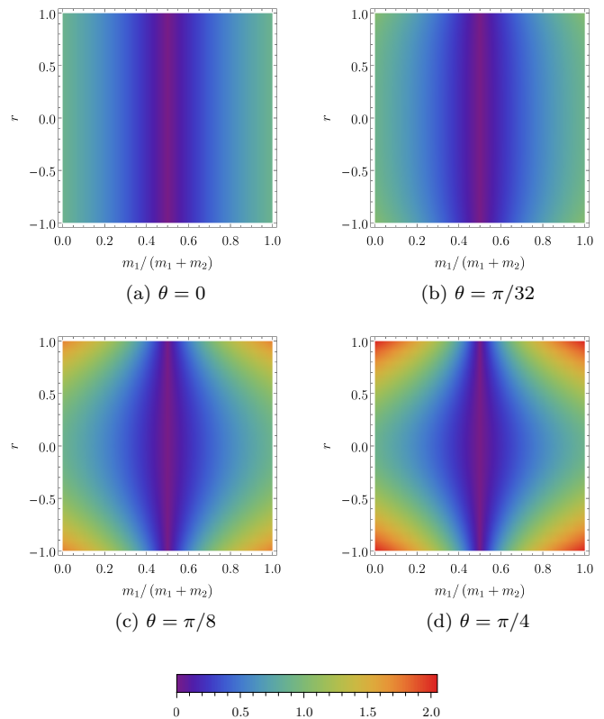
FIG. 1. (Colour online) The logarithmic negativity, as a measure of the entanglement between the center of mass and relation degrees of freedom, of the state associated with \mathbf{V}_{CMR} , when \mathbf{V}_1 = \mathbf{V}_2 and both \rho_1 and \rho_2 are pure, i.e. \det \mathbf{V}_1 = \det \mathbf{V}_2 = 1 , for different phase rotations \theta = \theta_1 = \theta_2 as a function of the squeezing parameter r = r_1 = r_2 and the ratio of masses m_1/(m_1 + m_2) .
