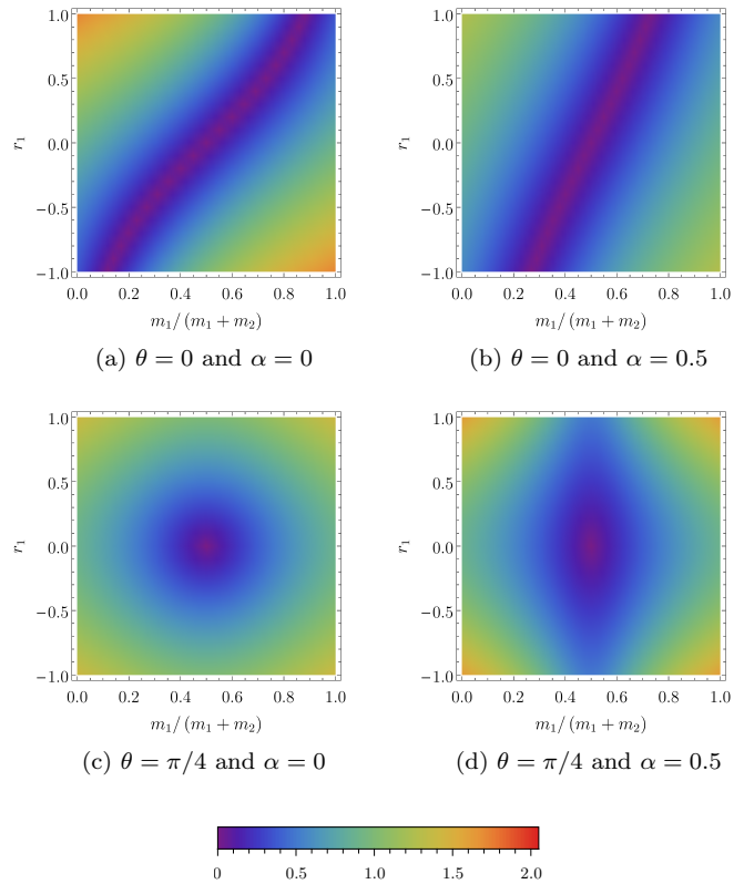
FIG. 3. (Colour online) The logarithmic negativity, as a measure of the entanglement between the center of mass and relation degrees of freedom, of the state associated with \mathbf{V}_{CMR} , when \det \mathbf{V}_1 = \det \mathbf{V}_2 = 1 for r_2 = \alpha r_1 , for different phase rotations \theta = \theta_1 = \theta_2 and values \alpha . Plots for \theta = 0 and \alpha = 1 and \theta = \pi/4 and \alpha = 1 are shown in Figs. 1a and 1d respectively.
