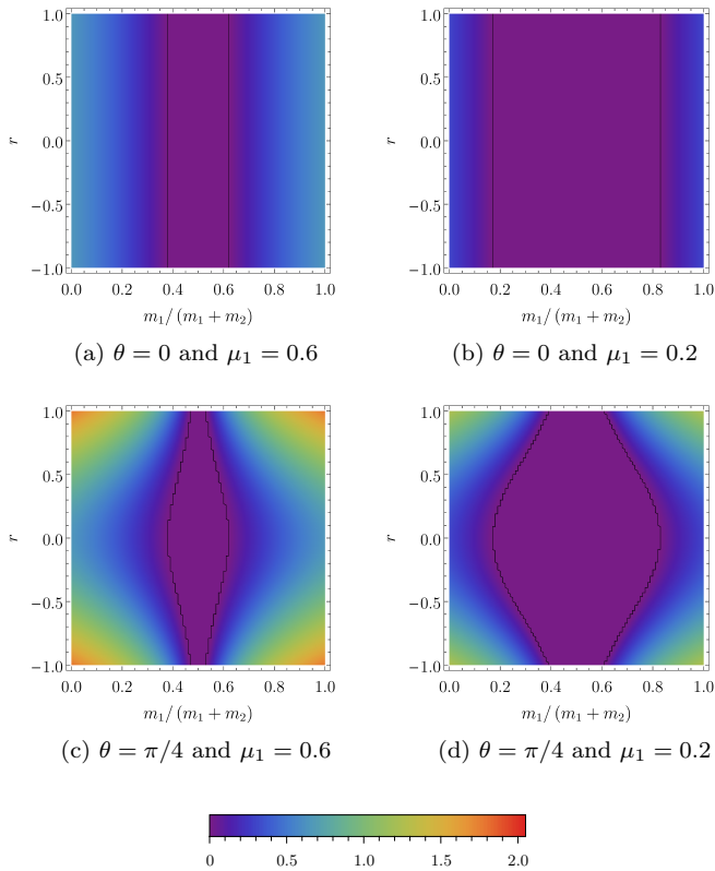
FIG. 2. (Colour online) The logarithmic negativity, as a measure of the entanglement between the center of mass and relation degrees of freedom, of the state associated with \mathbf{V}_{CMR} , when r = r_1 = r_2 , \theta = \theta_1 = \theta_2 , and particle 2 is a pure state \mu_2 = 1 and particle 1 is not, for different purities of particle 1 \mu_1 and phase rotations \theta . Plots for \theta = 0 and \mu = 1 and \theta = \pi/4 and \mu = 1 are shown in Figs. 1a and 1d respectively.
