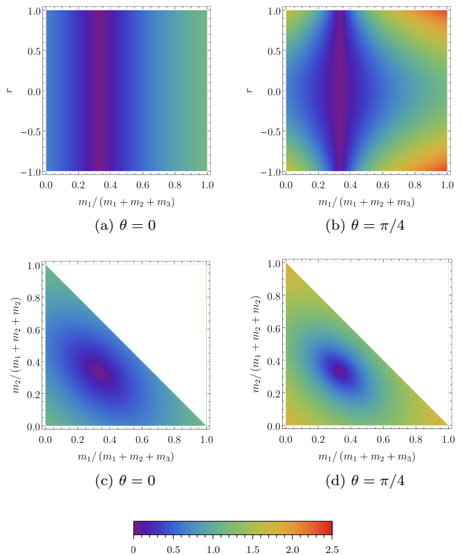
FIG. 4. (Colour online) The logarithmic negativity is plotted, as a measure of the entanglement between the center of mass and relation degrees of freedom, of the state associated with \mathbf{V}_{CMR} describing three particles. In (a) and (b) the logarithmic negativity is plotted for the case when m_2 = m_3 , for various equal phase rotations \theta_1 = \theta_2 = \theta_3 = \theta , as a function of the ratio m_1/(m_1 + m_2 + m_3) and equal squeezing parameter r_1 = r_2 = r_3 = r . In (c) and (d) the logarithmic negativity is plotted as a function of the two mass ratios m_1/(m_1 + m_2 + m_3) and m_2/(m_1 + m_2 + m_3) for various equal phase rotations \theta , with the equal squeezing parameter fixed at r = 0.7 .
