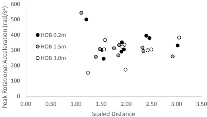
Peak Rot Accel (Ground) vs Scaled Distance
