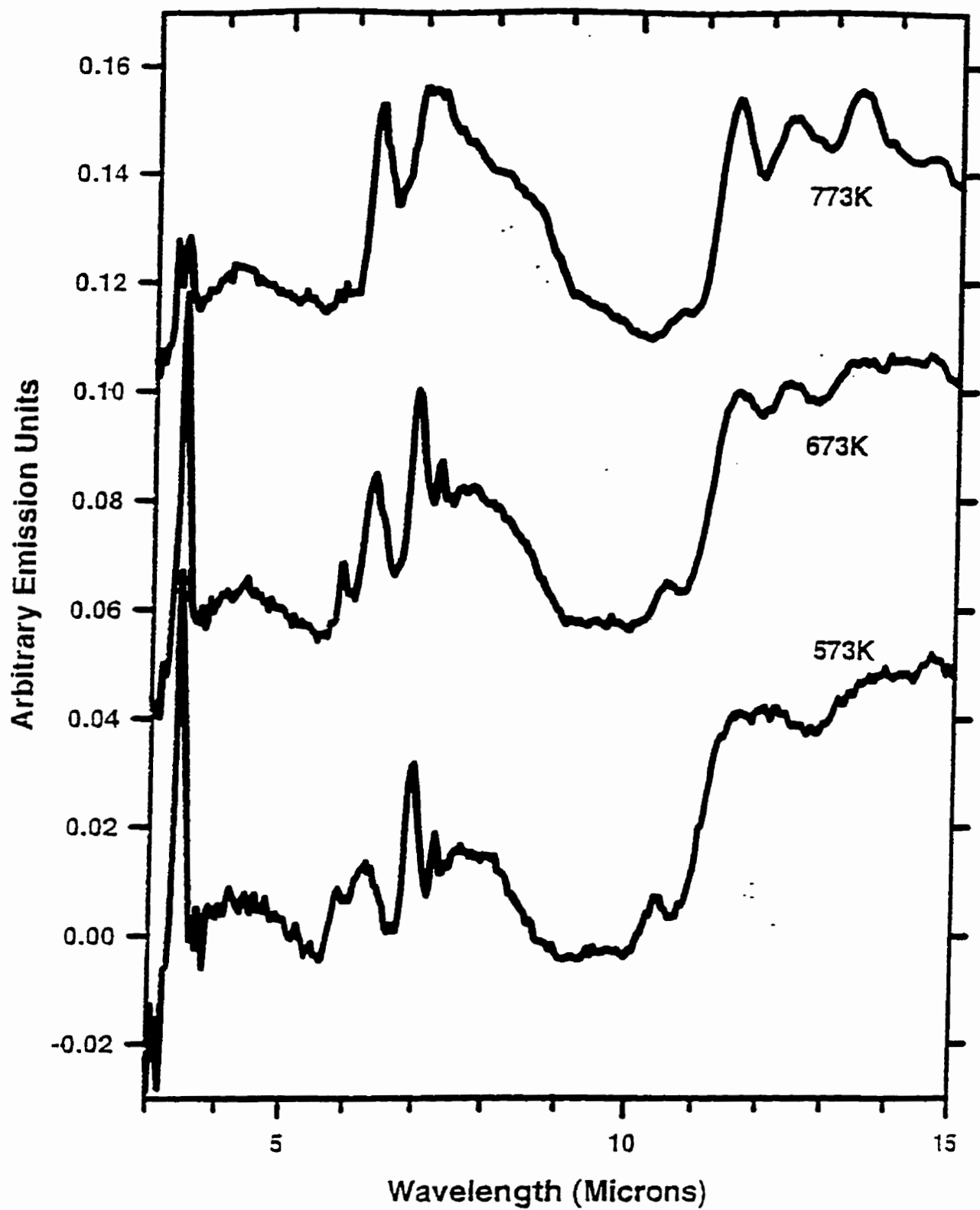
Figure 45 IR emission from HAC at various annealing temperatures (in vacuum) from 573-773K in the spectral range of 3-15 \mu m, zero shifted for clarity.
