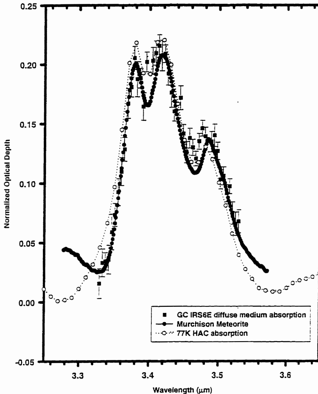
Figure 56 IR absorption spectrum of HAC deposited at 77K compared to astronomical observations of GC IRS6E and the Murchison Meteorite (Pendleton et al. 1994)
