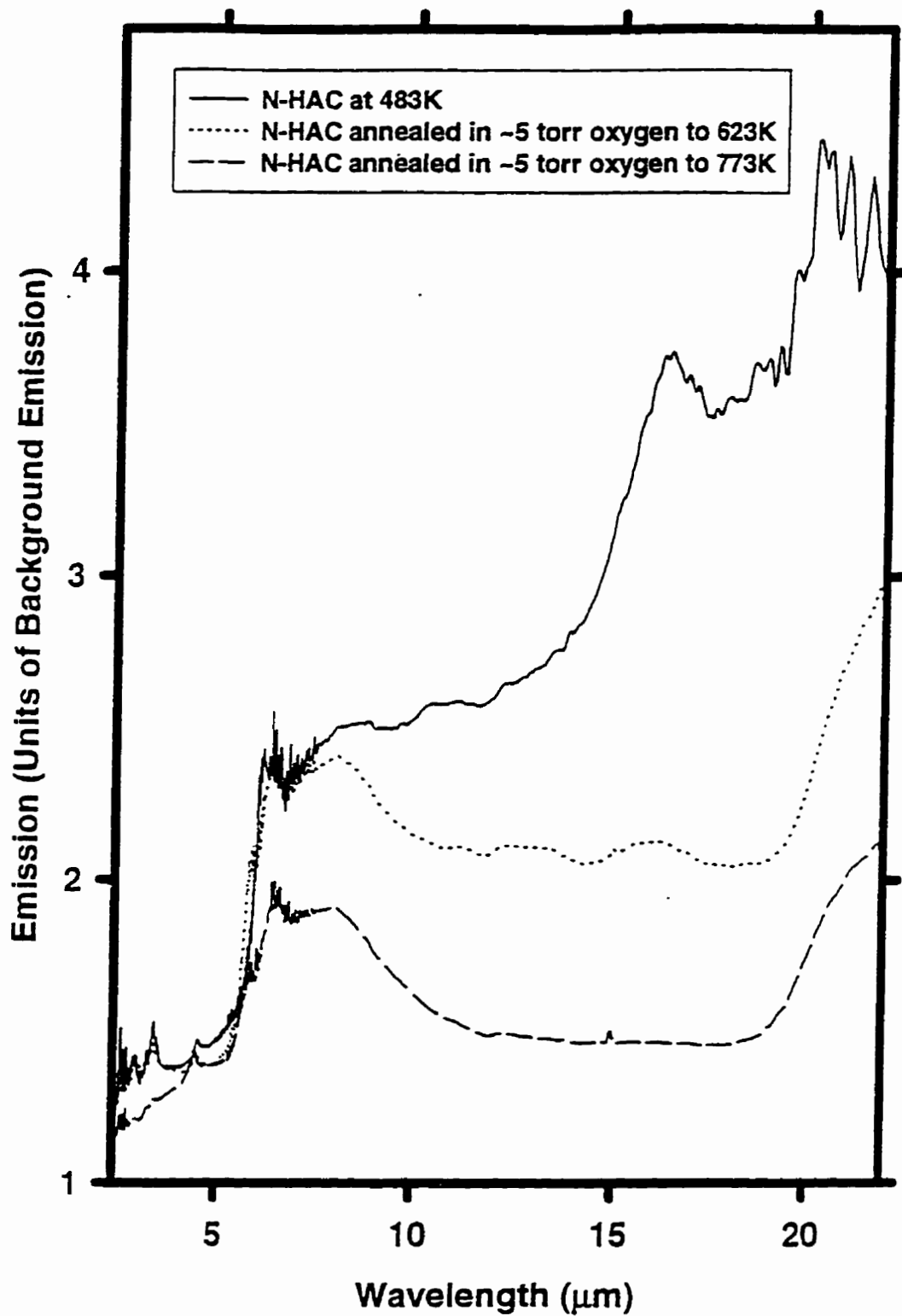
Figure 50 IR emission from N-HAC at 483K and annealed in oxygen to 623 and 773K.
