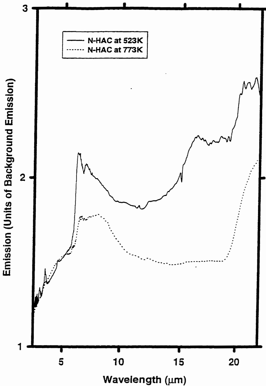
Figure 49 IR emission from nitrogenated HAC annealed in vacuum to 523 and 773K.
