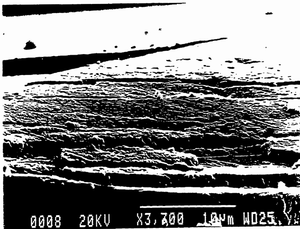
Figure 33 SEM of HAC film cross sections deposited at 300K: (a) as deposited; (b) photo-processed with UV radiation.
