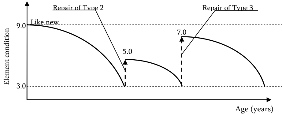
Figure 3.5: Condition Rating Improvement Model
