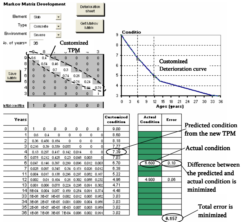
Figure 3.4: Optimized Markov Deterioration Matrix
