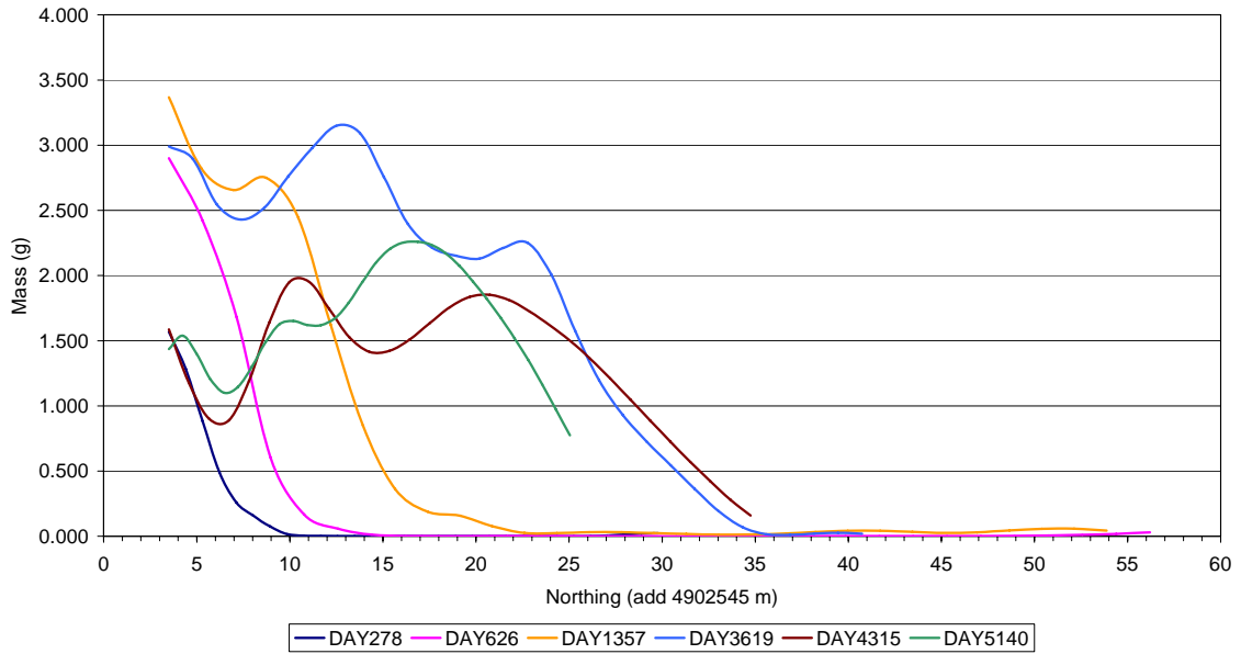
Acenaphthene - Longitudinal Distribution of Dissolved Mass
