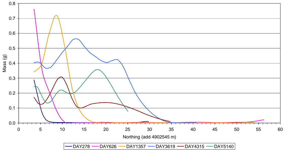
Carbazole - Longitudinal Distribution of Dissolved Mass
