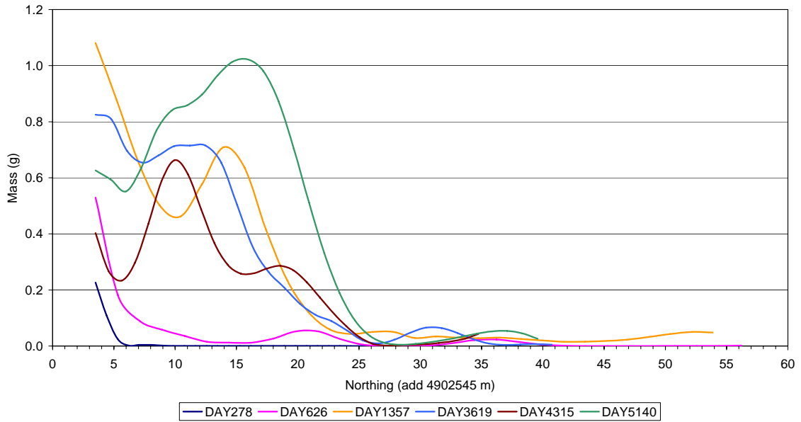
Fluorene - Longitudinal Distribution of Dissolved Mass
