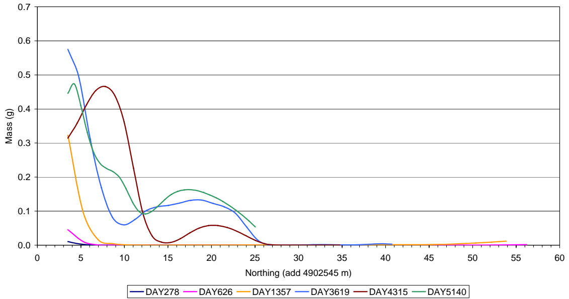
Phenanthrene - Longitudinal Distribution of Dissolved Mass
