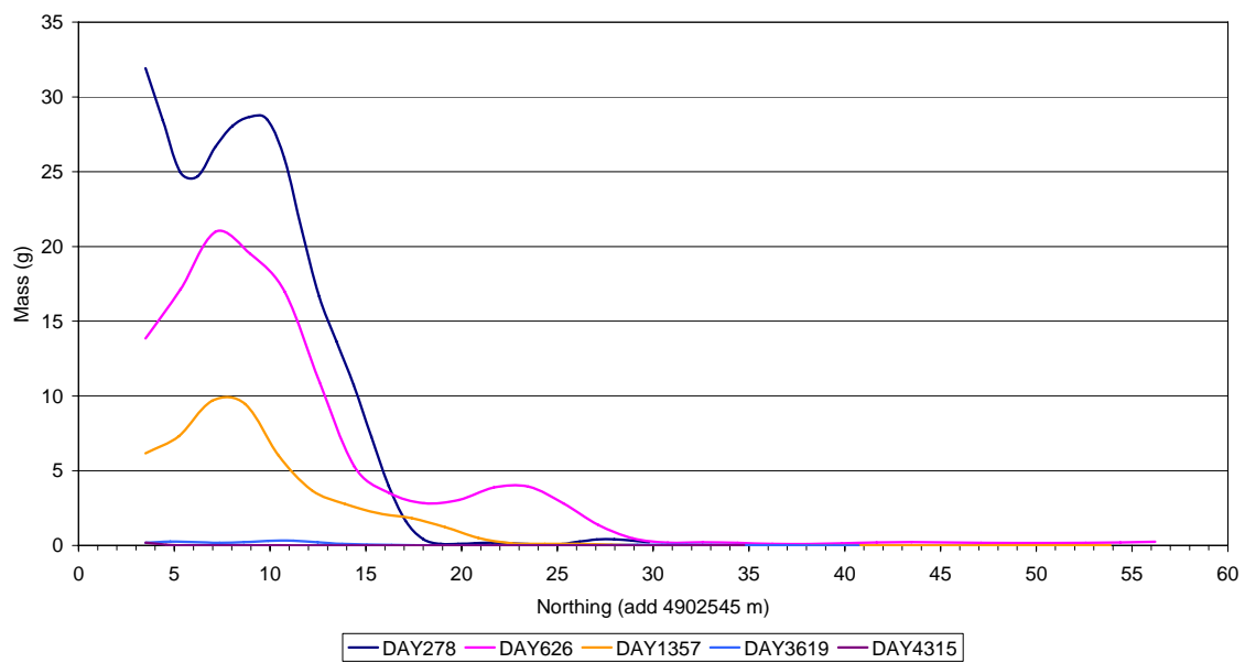
p+m-xylene - Longitudinal Distribution of Dissolved Mass
