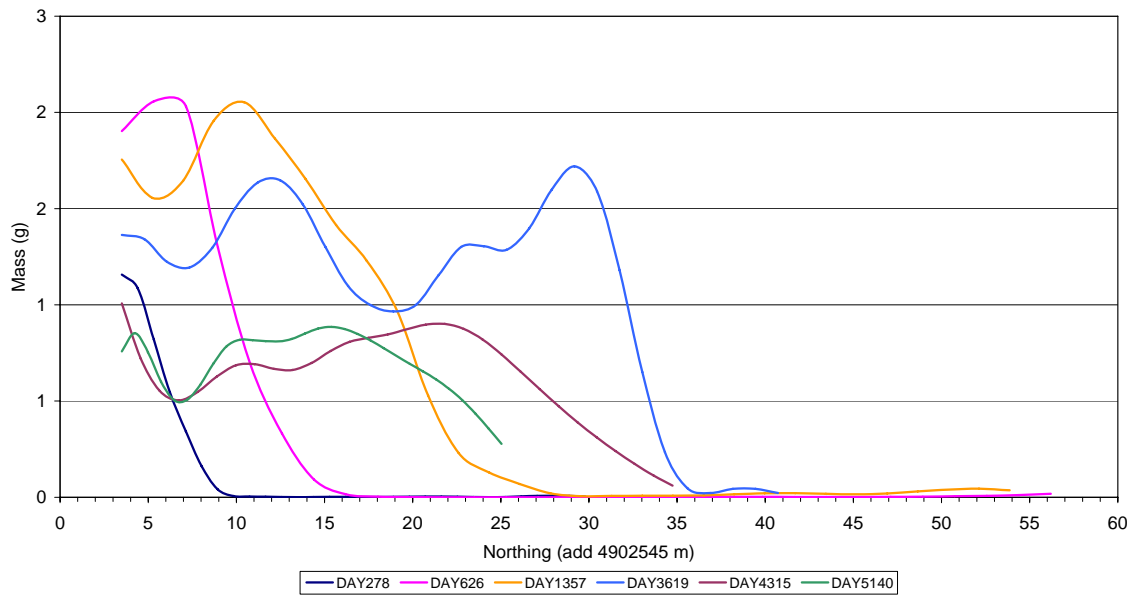
1-Methyl Naphthalene - Longitudinal Distribution of Dissolved Mass
