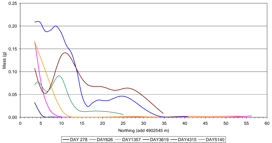
Anthracene - Longitudinal Distribution of Dissolved Mass
