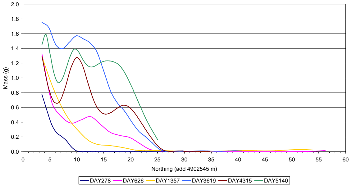
Dibenzofuran - Longitudinal Distribution of Dissolved Mass
