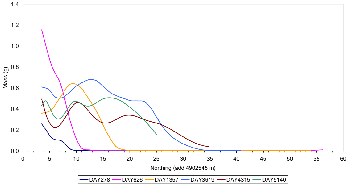
Biphenyl - Longitudinal Distribution of Dissolved Mass
