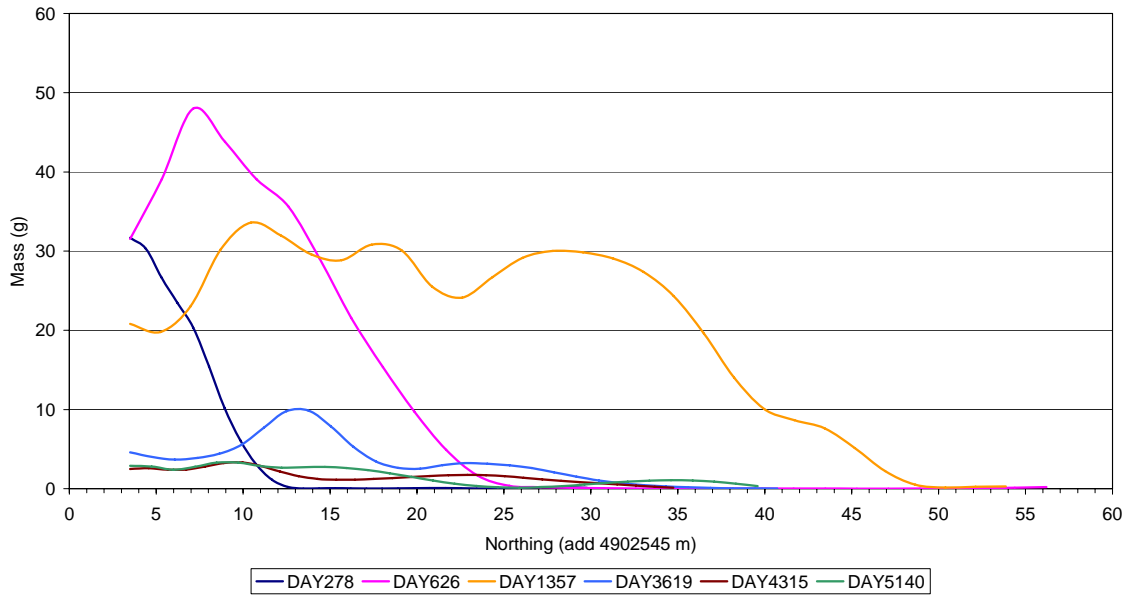
Naphthalene Plume - Longitudinal Distribution of Dissolved Mass
