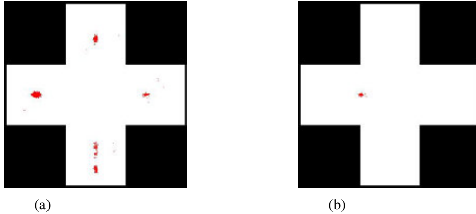
Figure 3-1: Global localization using ordinary MCL
