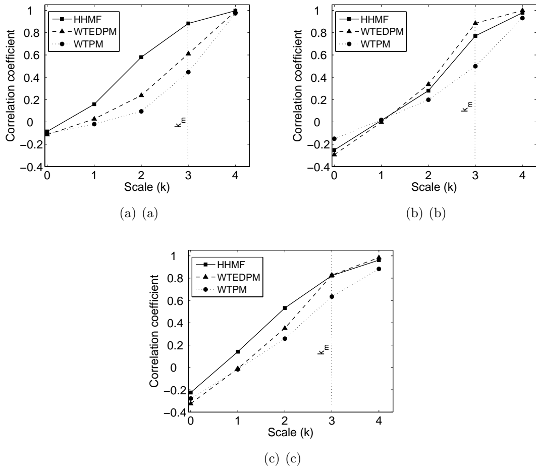
Figure 5.18: The correlation \rho_k between ground truth \hat{x}^* and reconstruction \hat{x} as a function of structure scale k for (a) a two-scale reconstruction from Fig. 5.10(a), (b) a fractal multi-scale reconstruction from Fig. 5.10(b), (c) a multi-model behaviour reconstruction from Fig. 5.10(c), where k_m denotes the resolution scale of the measurement, where k_m denotes the measurement scale. The proposed HHMF performs similarly to or better than the competing wavelet methods.
