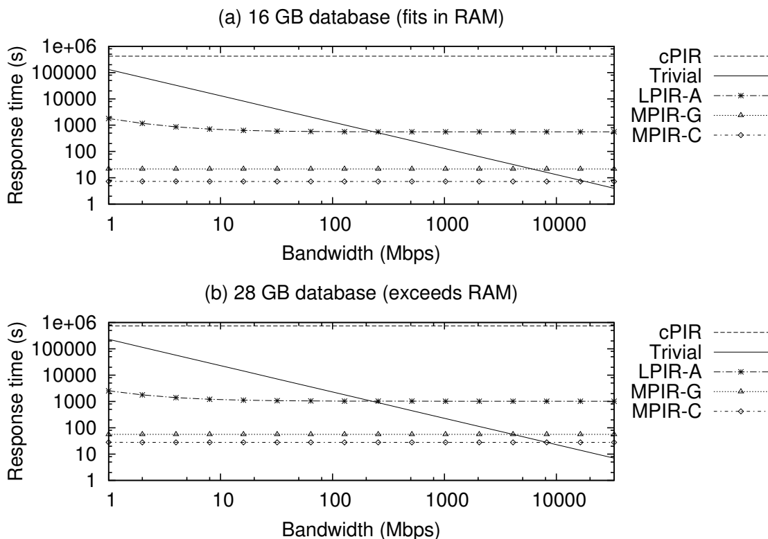
Figure 4.4: Plots of response time vs. bandwidth for the PIR schemes by Kushilevitz and Ostrovsky (cPIR) [KO97], Aguilar-Melchor [AMCG+08] (LPIR-A), Chor et al. [CGKS95] (MPIR-C) and Goldberg [Gol07a] (MPIR-G), as well as the trivial PIR scheme for database sizes that fit in RAM (16 GB) and that exceed RAM (28 GB).
