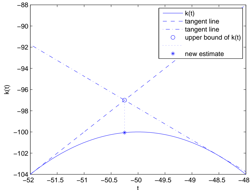
Figure 8: Triangle Interpolation
