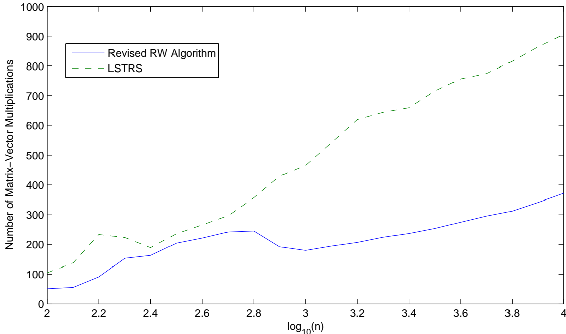
Figure 23: Revised RW vs LSTRS; Varying n ; Density= 0.01; Hard Case (Case 2)
