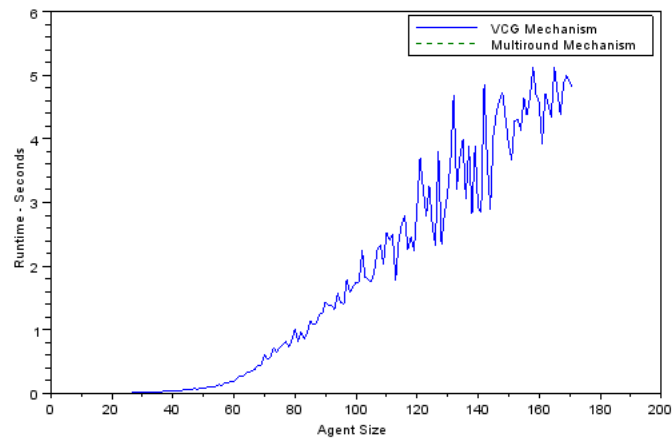
Figure 4.2: Runtime of the static mechanisms
