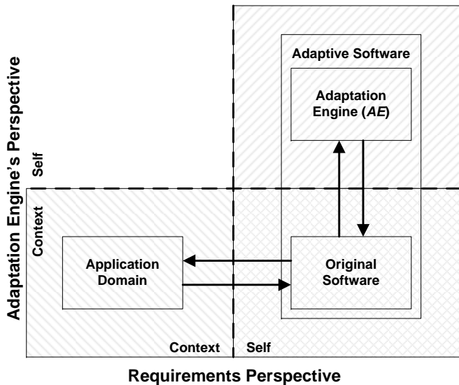
Figure 5.3: Problem of Finding a Mapping from Phenomena in the AD , Which are Described by the AR 's, to Their Corresponding Phenomena in the AS
