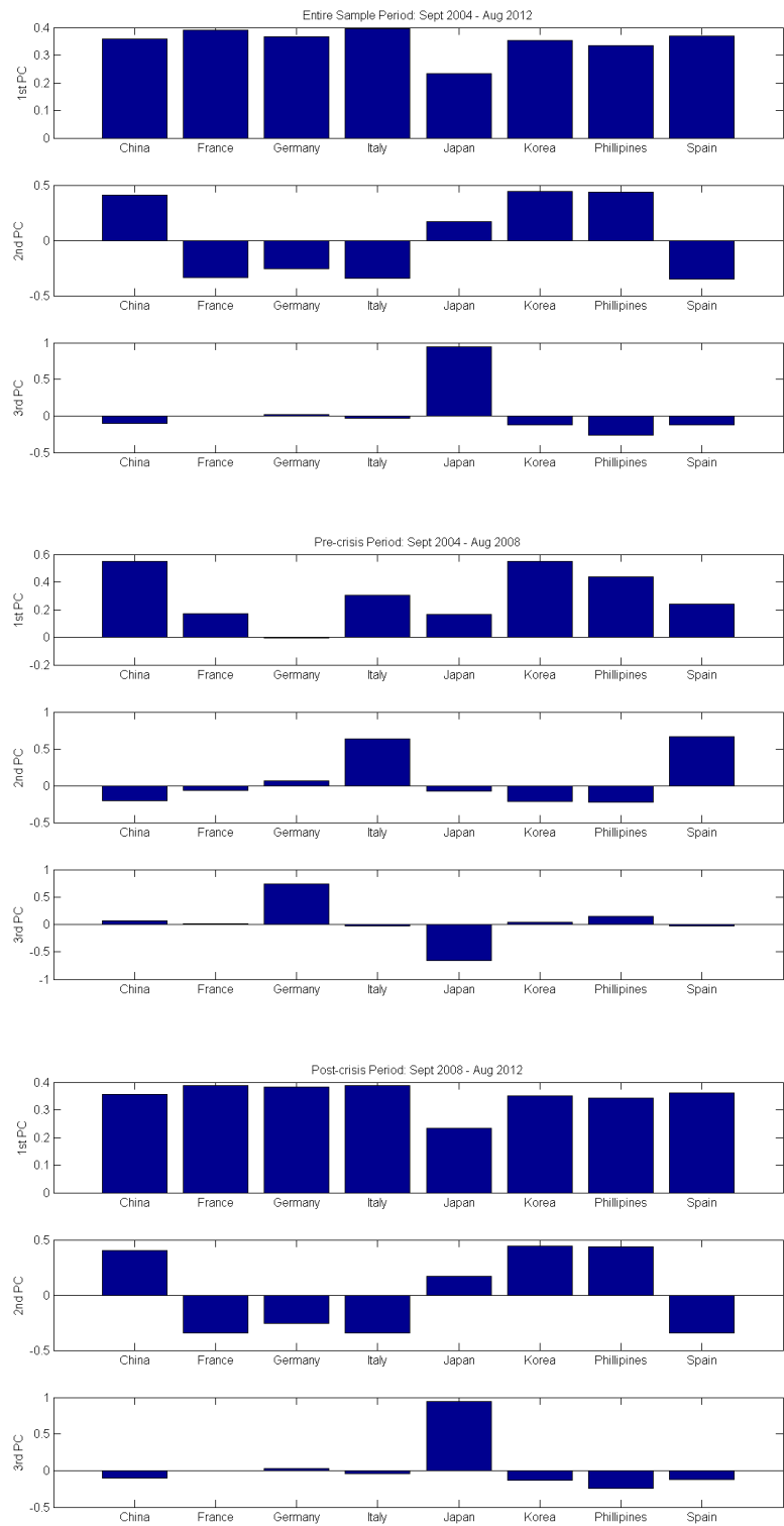
Figure 3.1: Loadings for First Three PCs of Daily Sovereign CDS Spreads Changes
